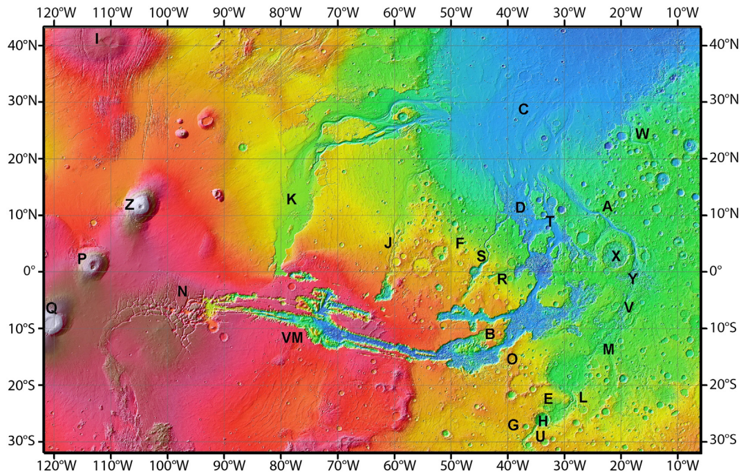
Fig. 22. Map of eastern Tharsis and circum-Chryse areas of Mars on MOLA topographic base (low areas in blue, high areas in red and brown). Features indicated by letters include volcanoes, I—Alba Patera, P—Pavonis Mons, Q—Arsia Mons, Z—Ascraeus Mons; impact basins and craters, C—Chryse, H—Holden; delta—Eberswalde; tectonic features, N—Noctis Labyrinthus, VM—Valles Marineris; channels and valleys, A—Ares, B—Columbia and Daga Valles, D—Simud Vallis, F—Nanedi Vallis, G—Nirgal Vallis, J—Maja Vallis, K—Kasei Vallis, L—Ladon Vallis, M—Morava Vallis, O—Osuga Vallis, R—Ravi Vallis, S—Shalbatana Vallis, T—Tiu Vallis, U—Uzboi Vallis, W—Mawth Vallis, X—Aran Chaos and channel, Y—Iani Chaos.
