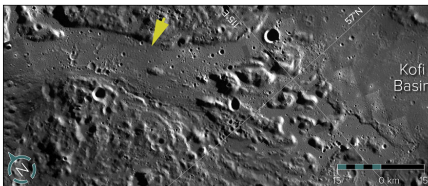
Fig. 2. Portion of the Mercury lava channel Angkor Vallis at 57^\circ \text{ N} latitude, 115^\circ \text{ E} longitude. The image is from the Mercury Dual Imaging System (MDIS) of the MESSENGER spacecraft and has a resolution of 250 m per pixel.
