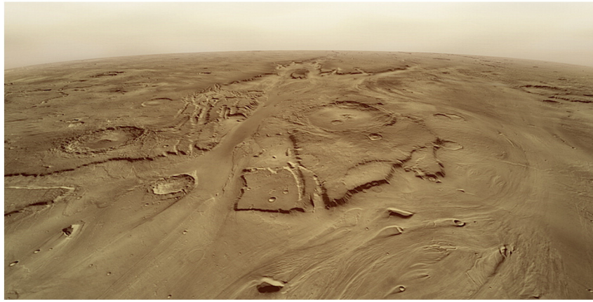
Fig. 23. Mouth of Kasei, the largest and longest (2400 km) “outflow channel” on Mars. This oblique view was generated at 2\times vertical exaggeration from the THEMIS data acquired by the Mars Odyssey spacecraft. The view is upstream, and the large crater in the center is Sharonov, which is 100 km in diameter. Note the splitting and convergence of channels (anastomosis).
