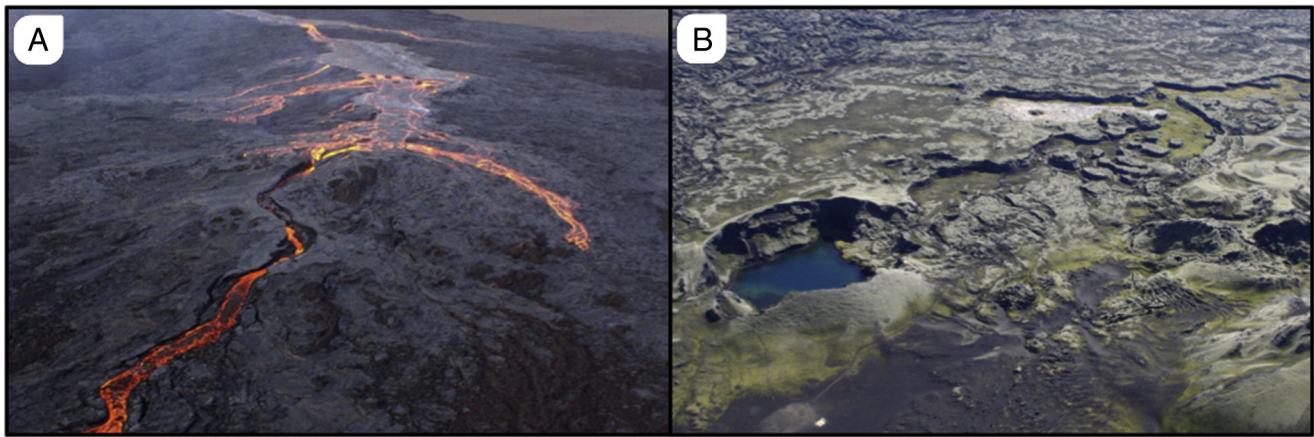
Fig. 20. Examples of terrestrial lava channels: (Left) example of an active lava channel forming on Kilauea, Hawaii, during the 2007–2008 phase of the Pu'u 'Ō'ō eruption; (Right) example of a 5-m-deep channel formed within the 1783–1784 A.D. Laki eruption in Iceland.
