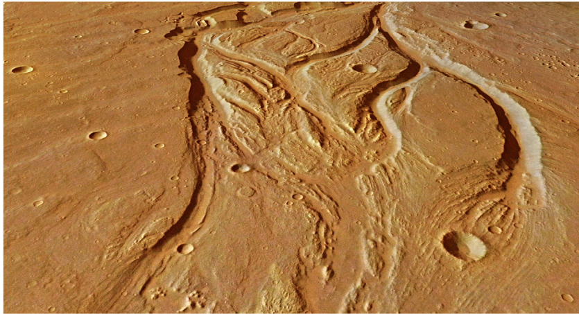
Fig. 25. Expansion bar complex in Osuga Vallis. This is an oblique view generated data provided by the High Resolution Stereo Camera (HRSC) on the Mars Express spacecraft. The view is downstream, and the channel width is about 20 km. The regional context for this image is shown in Fig. 29.
