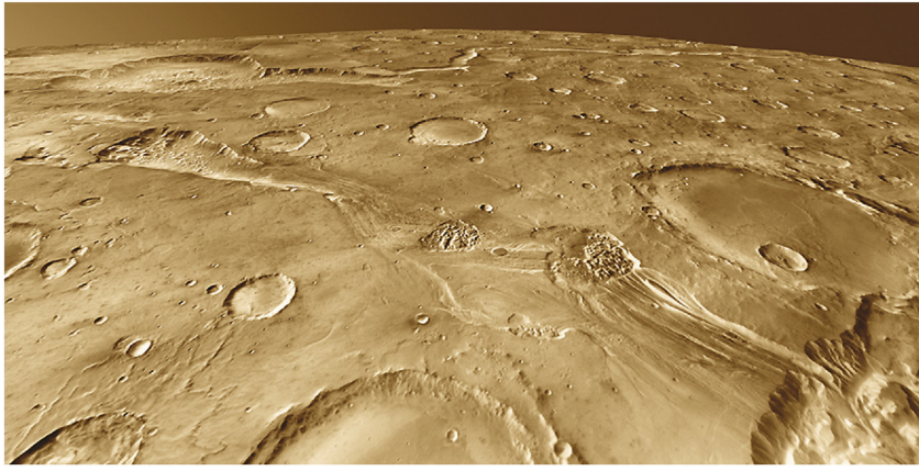
Fig. 27. Ravi Vallis. A 200-km long catastrophic flooding channel that emanates from Aromatum Chaos (left). Note the erosion of two chaos zones in the channel (center) and distal spilling of the channel-forming fluid over and the plateau edge to disappear into another chaos region (right foreground). This oblique view was generated from the Mars Odyssey spacecraft using the THEMIS instrument with a vertical exaggeration of about 1.5 \times .
