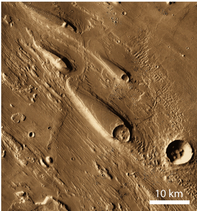
Fig. 24. Streamlined features in Ares Vallis (15.9° N, 330° E) imaged at visible wavelengths by the Thermal Emission Imaging System (THEMIS) on NASA’s Mars Odyssey orbiter. The cataclysmic flooding came from the lower right. Lins is the post-flooding, fresh looking crater in the lower right. It is about 6 km in diameter, and the imaged scene is about 40 \times 50 km. The streamlined features probably developed by a combination of deposition and preservation of pre-flood bedrock downstream from obstructions to the cataclysmic flood flows. There are also smaller-scaled lineated forms that may have developed as grooves or as depositional accumulations behind small obstructions. They are oriented longitudinally relative to the cataclysmic flood flows. Some intriguing transverse bedforms occur in the upper left quadrant of the image. These have orientations similar to what would be expected for subfluvial dunes, but at a spacing of about 500 m they are even larger than would occur in terrestrial cataclysmic flooding channels. North is up in the figure.
