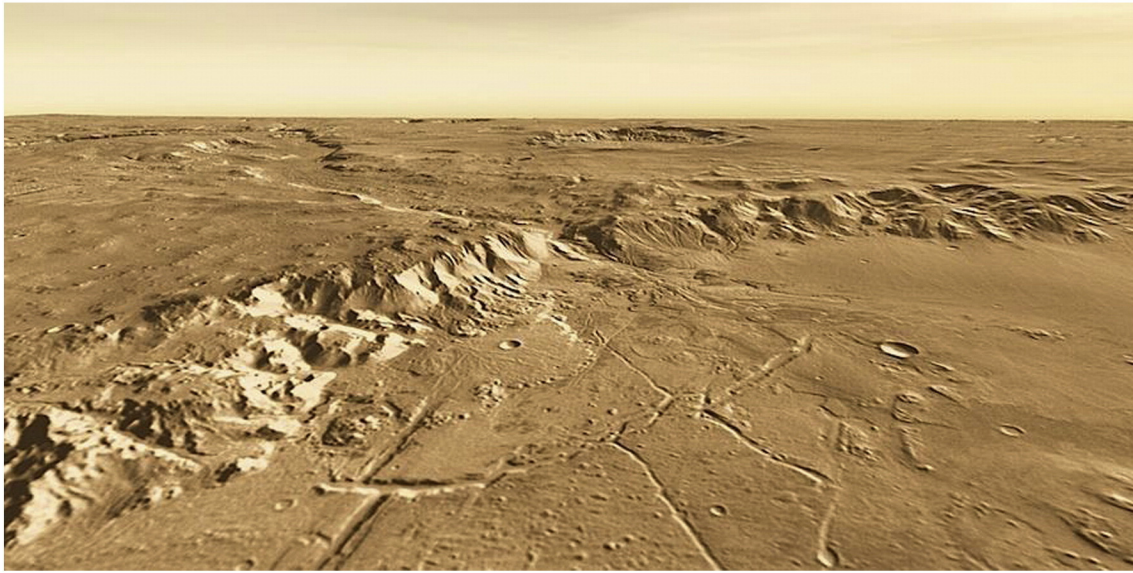
Fig. 30. Oblique view with a 2\times vertical exaggeration of a portion of the Uzboi–Ladon–Margaritifer (ULM) system generated from visible THEMIS data acquired by the Mars Odyssey spacecraft. The view is toward the southwest, showing the mouth of Uzboi Vallis (center) into Holden Crater through its southern rim. There is a fan-like accumulation of layered sediments at this junction, and a possible landing site for the Mars Science Laboratory rover was proposed for the flat, smooth area at right center, close to where the channel cuts through the rim.
