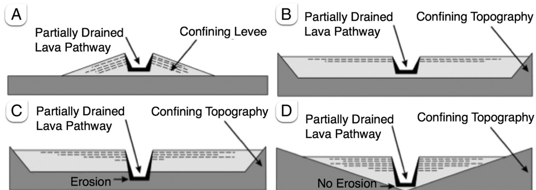
Fig. 19. Lava channel formation scenarios: (A) partially drained channel bounded by confining levees; (B) broad sheet-like lava lobe bounded by the initial topography; (C) deep channel formed by thermal-mechanical erosion into the substrate followed by partial drainage of the preferred lava pathway; (D) deep channel formed by constructional processes followed by lava drainage without substrate erosion.
