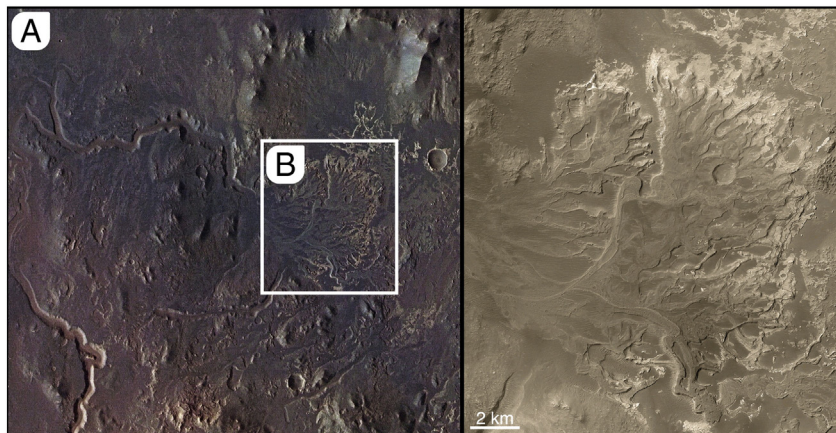
Fig. 13. (A) Image of Eberswalde delta taken by the High-Resolution Stereo Camera (HRSC) of the Mars Express spacecraft. The delta surface is marked by alluvial paleochannels that fed into a lake that occupied the Eberswalde crater. The inset (B) shows the location of the figure on the right. Right: Detail of the distributary complex of alluvial channels imaged by the Mars Orbiter Camera (MOC). The channel sediments, presumably sand and/or gravel, are etched into positive relief because of the erosional removal of adjacent materials, presumably overbank silt and/or clay. Note the prominent scroll bar topography associated with the meander bend near the center of the image. North is up in each figure.
