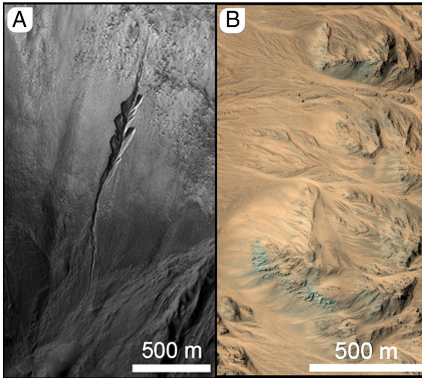
Fig. 16. (A) A portion of Mars Reconnaissance Orbiter (MRO) High Resolution Imaging Science Experiment (HiRISE) image PSP_1712_1405 (0.3 m/pixel resolution) showing theater headed gully tributaries with inner channels (left). Sun direction is from the left, and north is up. (B) Portion of HiRISE image PSP_001415_1877 (0.3 m/pixel resolution). The image shows the eastern rim region of Mojave crater, which is extensively dissected by integrated gully systems. North is up in the figure, and the sun is illuminating from the left.
