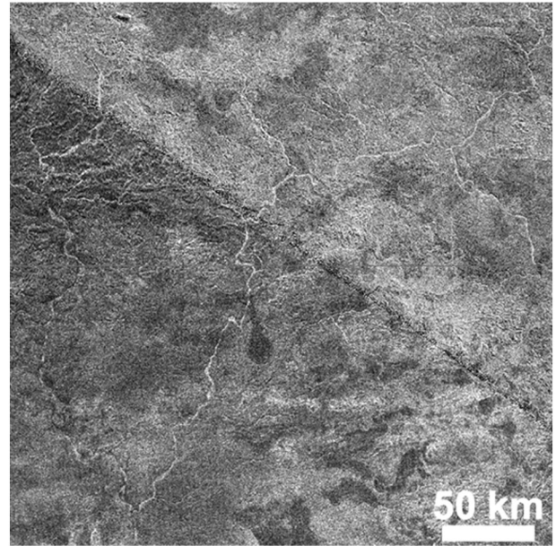
Fig. 7. Mosaic of synthetic aperture radar (SAR) images from the Titan Radar Mapper of the Cassini Mission, showing narrow, elongate fluvial valleys in the Xanadu region, approximately 100° S, 1370° W on Titan. On this image, fluvial features are bright, which is hypothesized for other radar-bright fluvial features to result from internal reflections from cobble-sized debris. SAR image quality varies across the mosaic. North is up in this figure. Image courtesy of National Aeronautics and Space Administration (NASA)/Jet Propulsion Laboratory (JPL)/European Space Agency (ESA)/U. Arizona.
