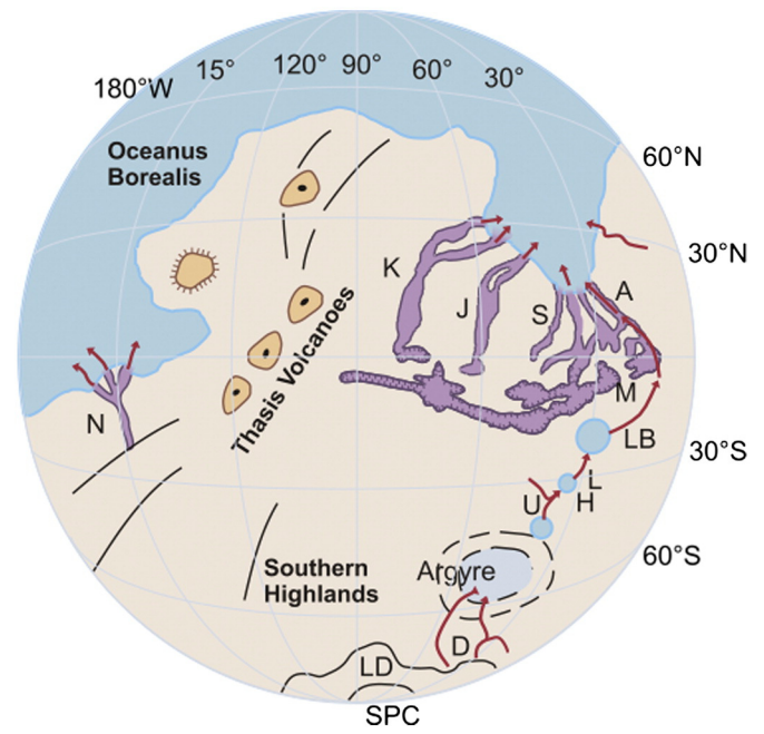
Fig. 29. Sketch map of the western hemisphere of Mars, showing the 8000 km drainage system, including the Uzboi–Ladon–Margaritifer (ULM) system, that extends to the northern plains ('Oceanus Borealis') from the layered deposits (LD) that underlie the South Polar Cap (SPC). Elements of the drainage include (from south to north): Dzigai Vallis (D), the Argyre impact basin, Uzboi Vallis (U), Holden Crater (H), Ladon Vallis (L), Ladon Basin (LB), Margaritifer Vallis (M), and Ares Vallis (A). Other prominent cataclysmic flooding channels include Mangala Vallis (N), Kasei Vallis (K), Maja Vallis (J), and Shalbatana Vallis (S).
