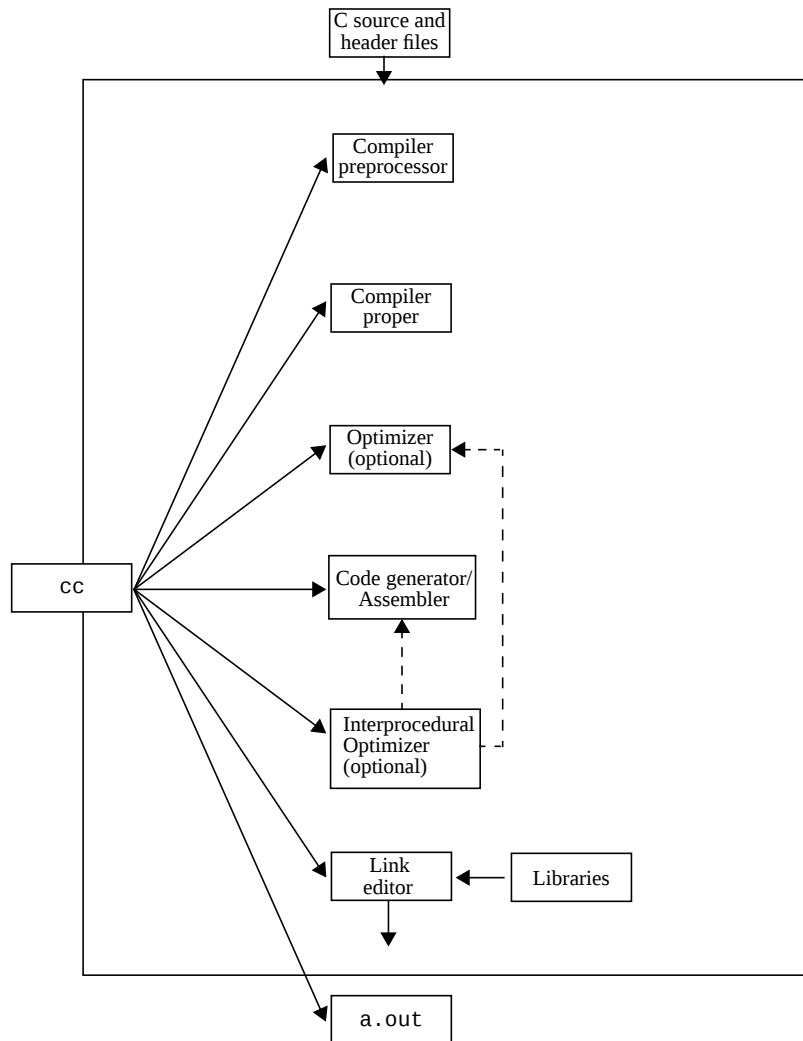
FIGURE 1-1 Organization of the C Compilation System
